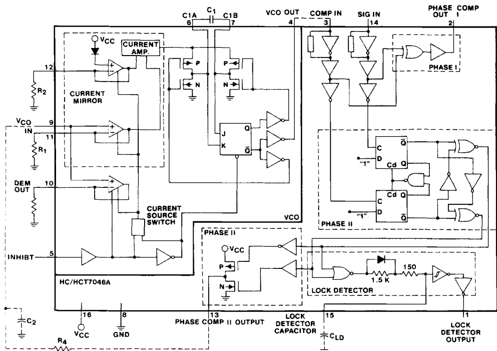
Fig. 1 - Logic diagram.
