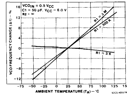
Fig. 24 - HC7046A typical change in VCO frequency vs. ambient temperature as a function of R_1 .
