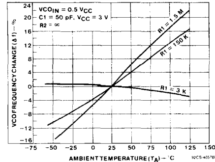
Fig. 22 - HC7046A typical change in VCO frequency vs. ambient temperature as a function of R_1 ( V_{CC}=3\text{ V} ).
