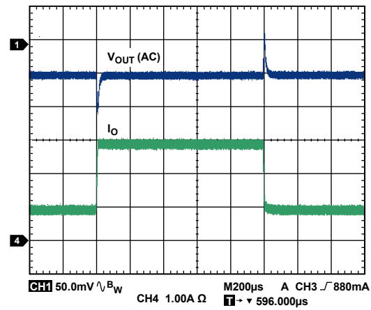
Figure 9. Load Transient (ADP2119, FPWM, V_{IN} = 5V , V_{OUT} = 1.2V )
