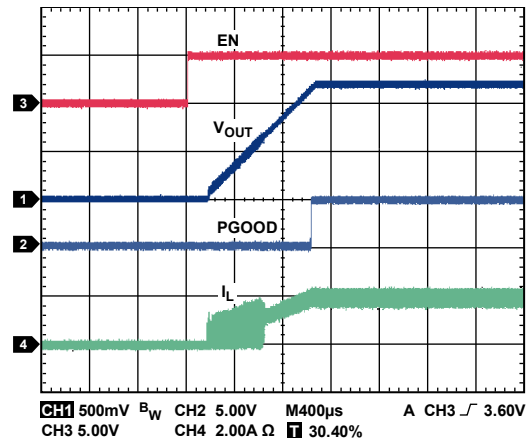
Figure 8. Soft Start (ADP2119, V_{IN} = 5V , V_{OUT} = 1.2V )
