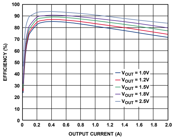
Figure 5. ADP2119 Efficiency, V_{IN} = 3.3V , FPWM
