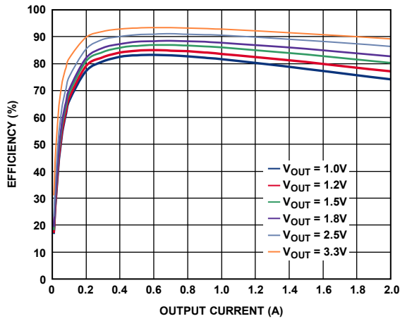
Figure 4. ADP2119 Efficiency, V_{IN} = 5V , FPWM
