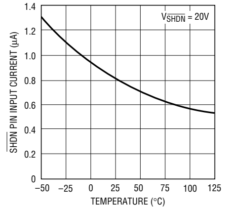
SHDN1 or SHDN2 Pin Input Current
