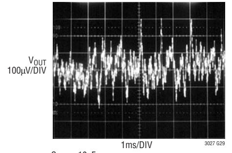
10Hz to 100kHz Output Noise C_{\text{BYP}} = 100\text{pF}
