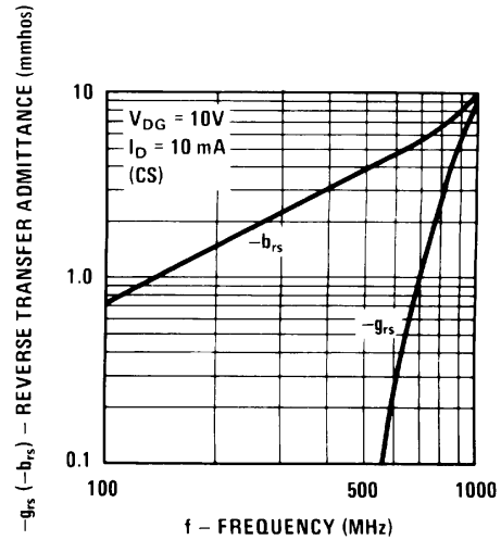
Figure 15. Reverse Transadmittance
