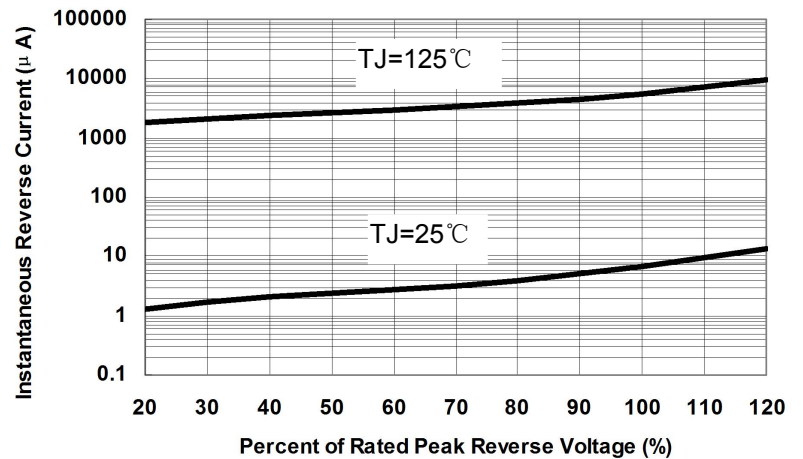
Fig.2-Typical Reverse Characteristics
