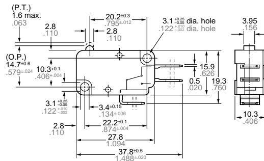
.187 Quick-connect/Solder terminal
