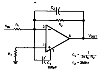
Figure 3. Feedforward Compensation
