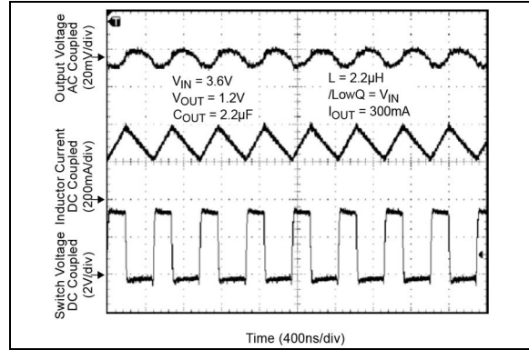
FIGURE 2-27: DC/DC PWM Waveforms.
