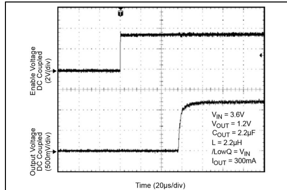
FIGURE 2-29: DC/DC Start-Up Waveforms.
