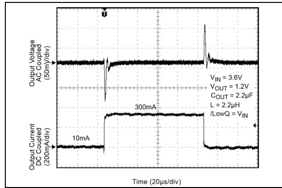
FIGURE 2-28: DC/DC Load Transient.
