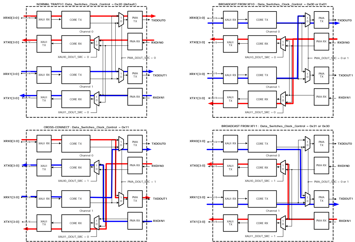
Figure 19 • Cross-Connect Configuration
