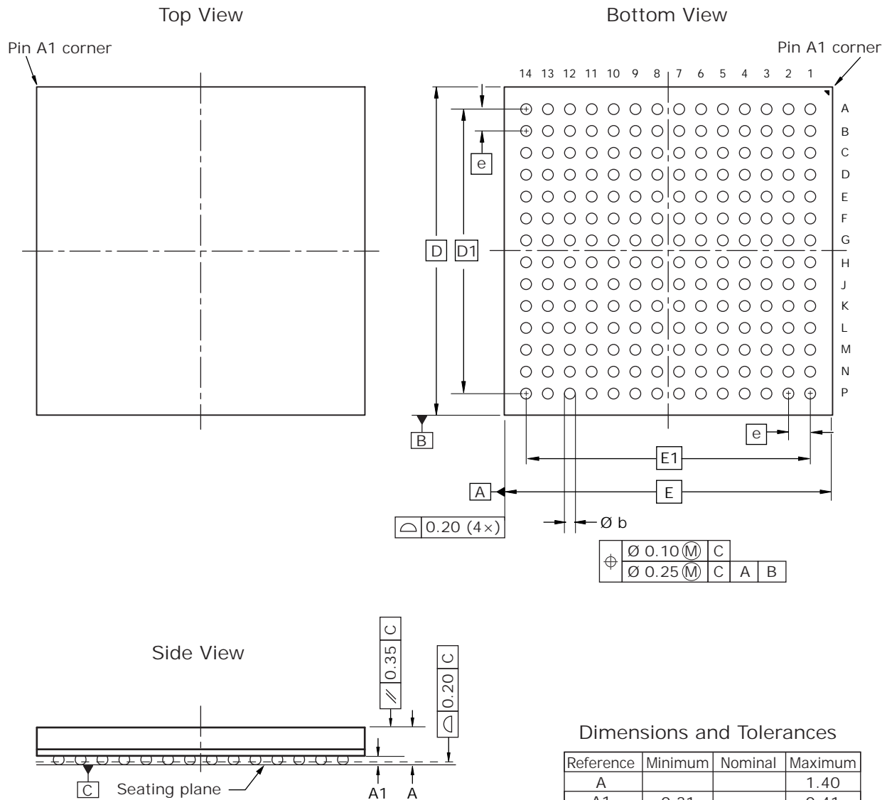
Figure 46 • Package Drawing
