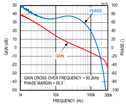
CONDITIONS: PWM MODE, 4.25A LOAD
