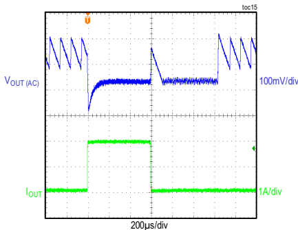
CONDITIONS: PFM MODE
