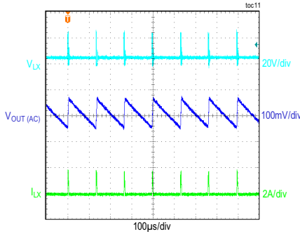
CONDITIONS: PFM MODE, 50mA LOAD
