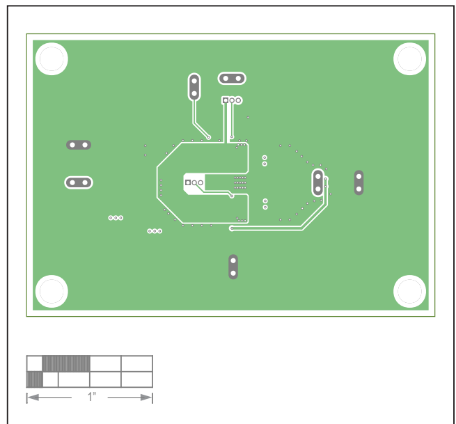
MAX17634B EV Kit—Layer3 GND
