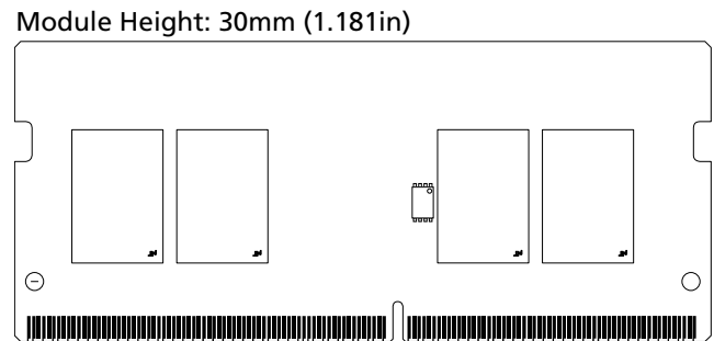
Figure 1: 260-Pin SODIMM (R/C A1, R/C A2)
