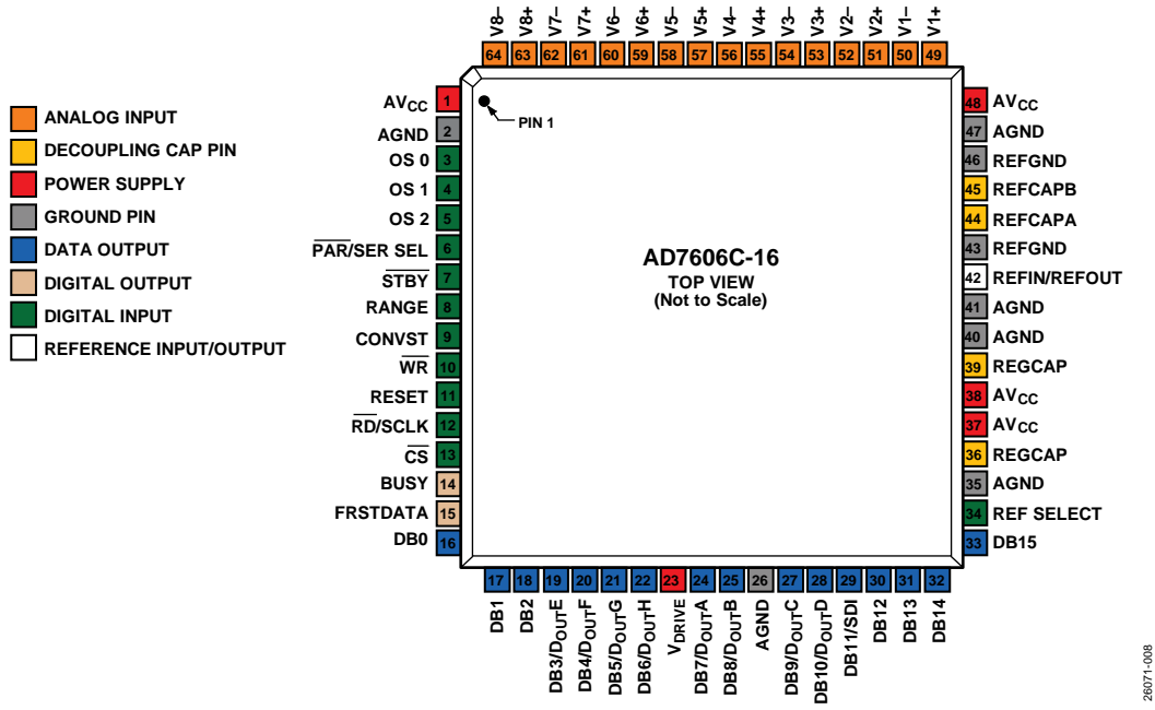
Figure 8. Pin Configuration
