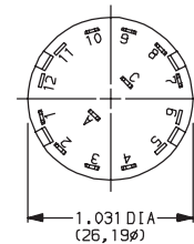
TERMINAL NOS. MOLDED ON HOUSING
