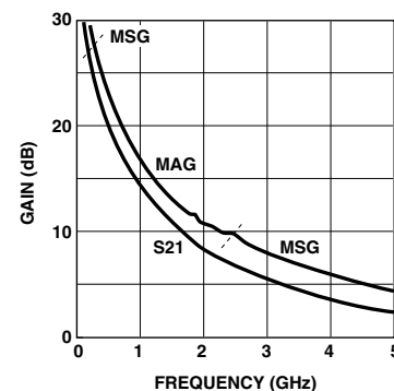
Figure 22. AT-32033 Gains vs. Frequency at V_{CE} = 2.7 V , I_C = 20 mA .
