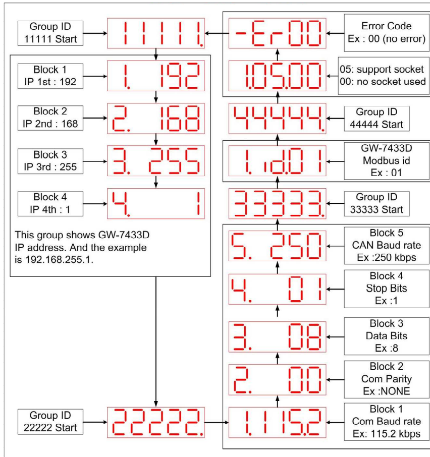
Figure 2: The meaning of the 7-segment LED
