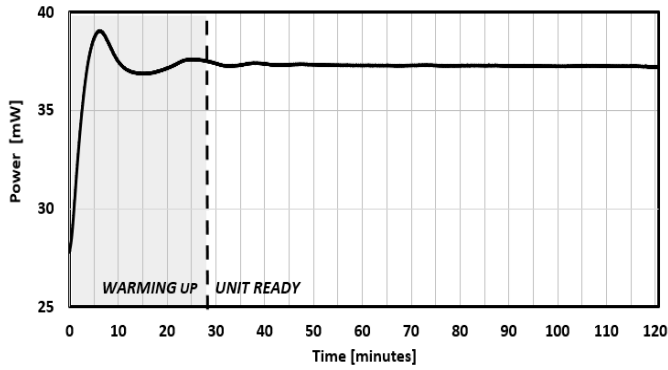
FIG. 7: WARM-UP TIME
