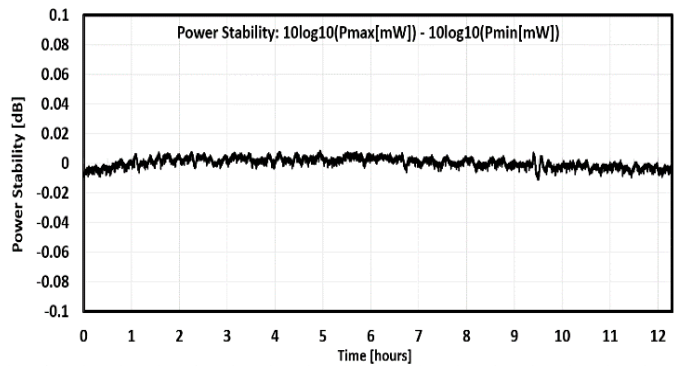
FIG. 6: ISB2 TYPICAL POWER STABILITY
