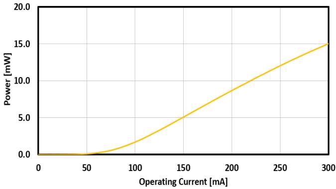
FIG. 5: SLED 2 OUTPUT POWER VS CURRENT
