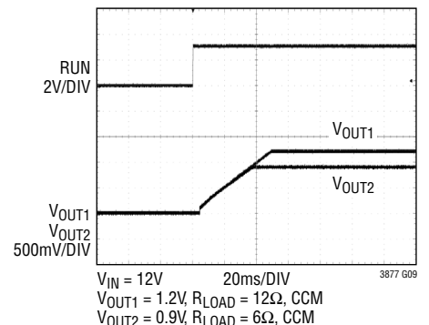
Coincident Tracking
