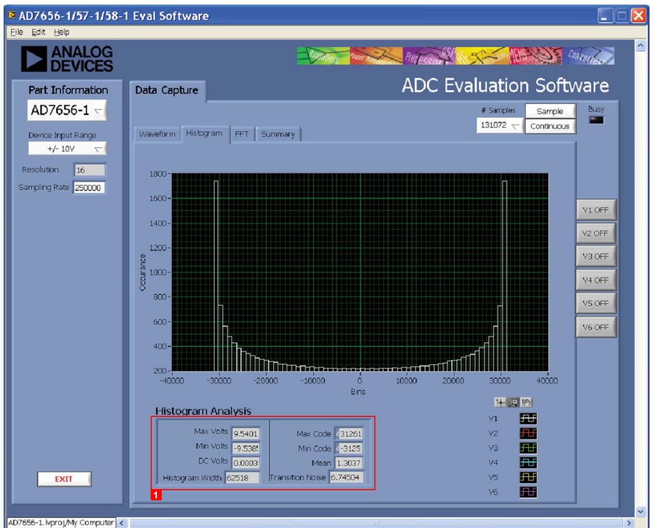
Figure 19. Histogram Tab
