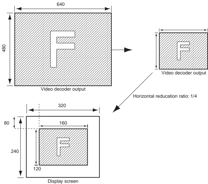
Figure J.2 Interlace Composite Capture (Horizontal and Vertical Reduction Ratios = 1/4)
