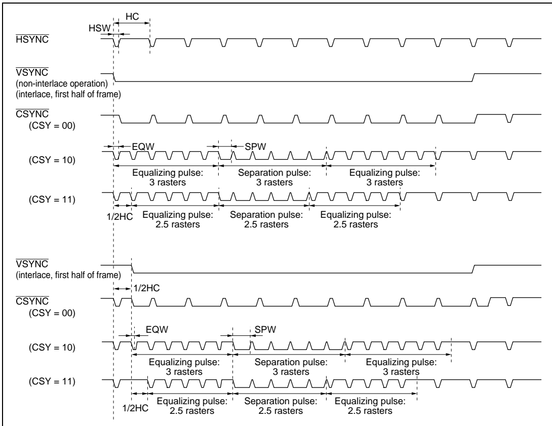
Figure 3.37 \overline{\text{CSYNC}} Output Waveform
