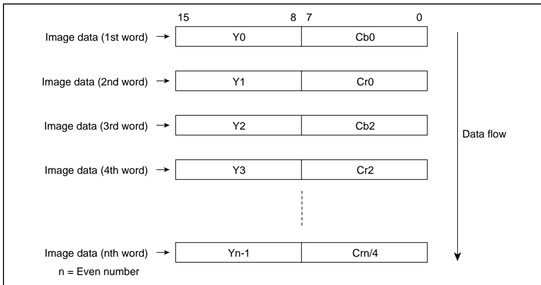
Figure 3.65 The Flow of YCbCr (4:2:2) Data
