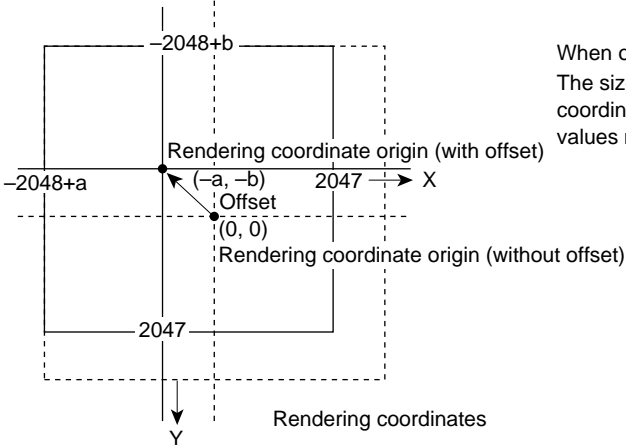
Figure 3.16 Rendering Coordinates
