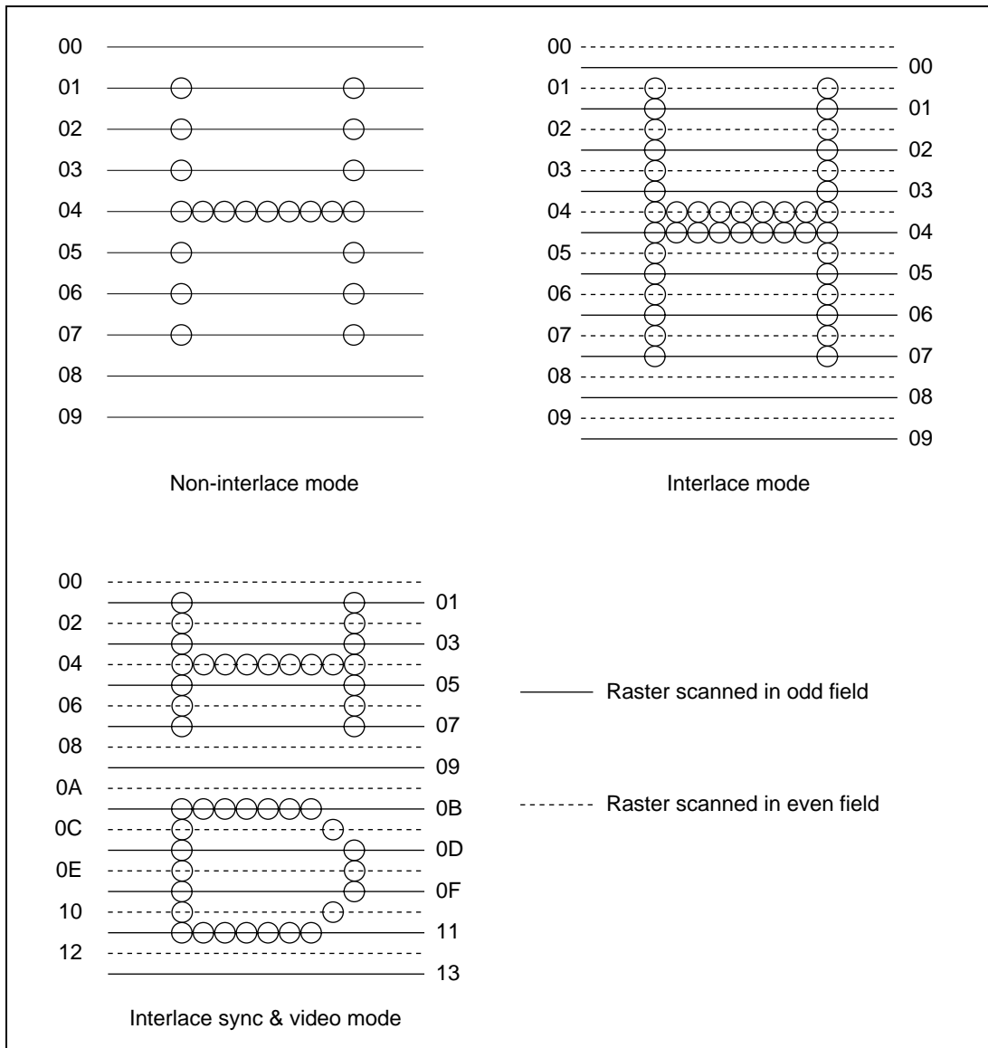
Figure 3.29 Examples of Raster Scan Control Display
