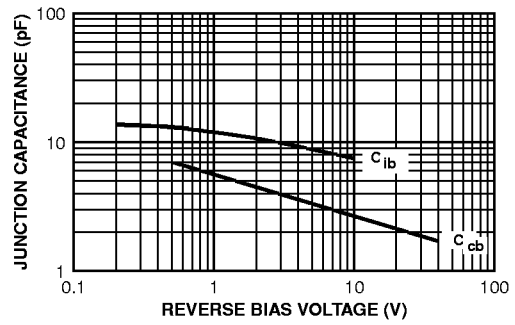
Junction Capacitance vs Reverse Bias Voltage
