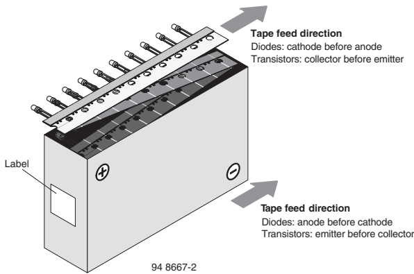
Fig. 22 - Tape Direction
