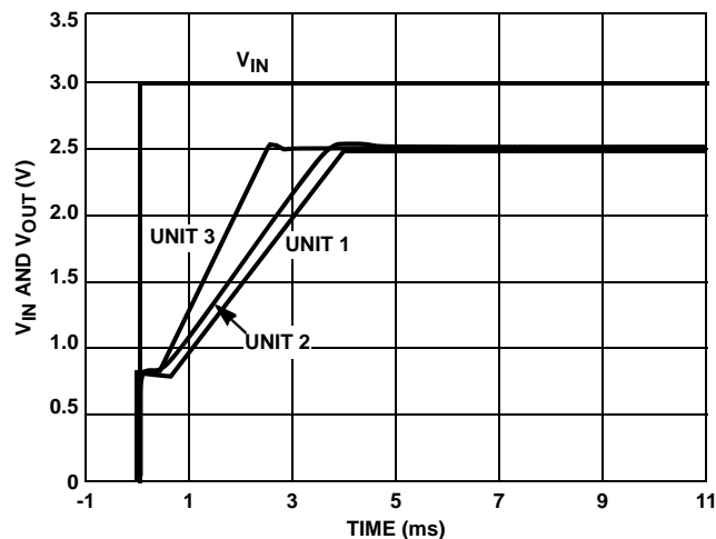
FIGURE 119. TURN-ON TIME
