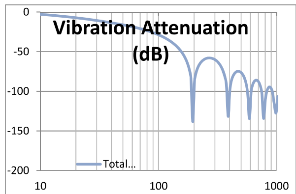
Attenuation vs. Vibration Frequency Fclk = 100kHz
