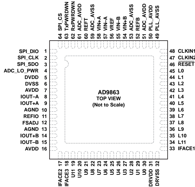
Figure 3. Pin Configuration
