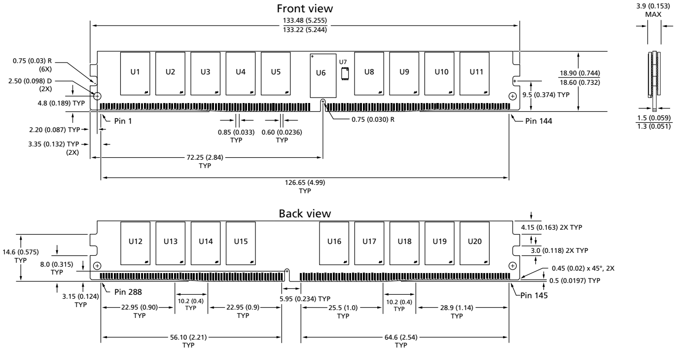
Figure 5: 288-Pin DDR4 VLP RDIMM (PCB 2954)
