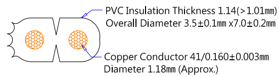
SPT-2 18AWGx2C 截面圖 (Wire Cross-Section)
