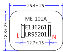
ME-101A (NEMA 1-15P) (Dimensions of Plug Face)
