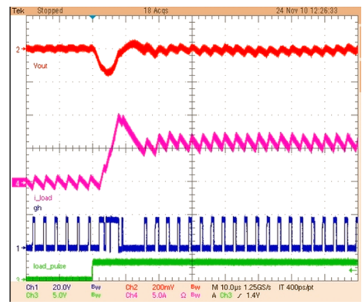
Figure 4: 0-6A Transient 300kHz with OVS +/-5%
