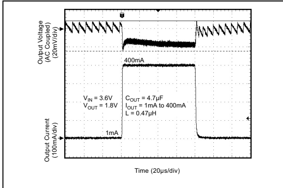
FIGURE 2-25: Load Transient.
