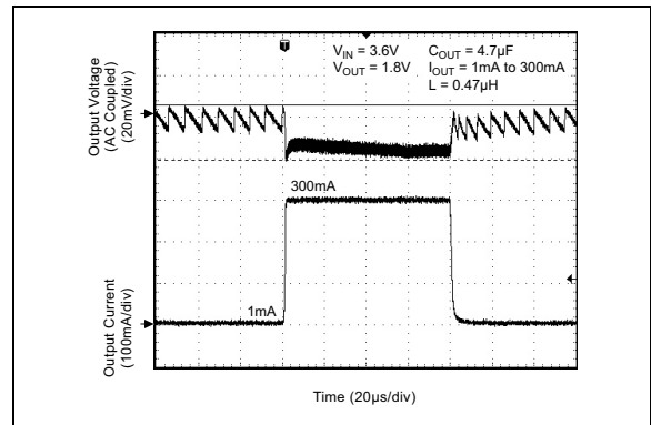
FIGURE 2-24: Load Transient.
