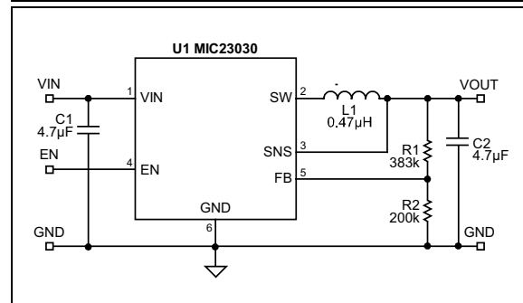
FIGURE 4-1: MIC23030-AYMT Schematic.
