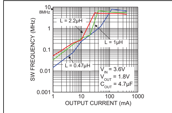
FIGURE 2-10: Switching Frequency vs. Inductance.
