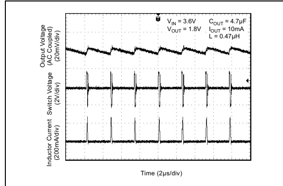
FIGURE 2-16: Switching Waveform - Discontinuous Mode.
