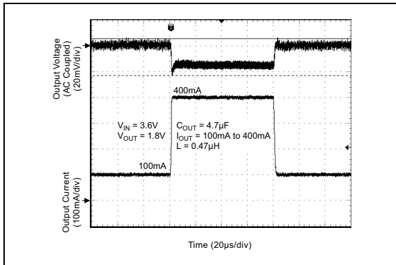
FIGURE 2-26: Load Transient.
