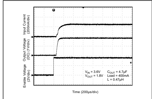
FIGURE 2-22: Start-Up Waveform.
