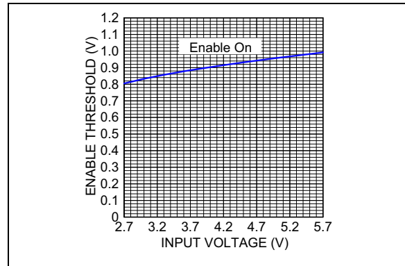
FIGURE 2-12: Enable Threshold vs. Input Voltage.
