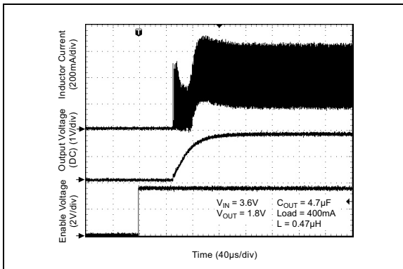
FIGURE 2-21: Start-Up Waveform.
