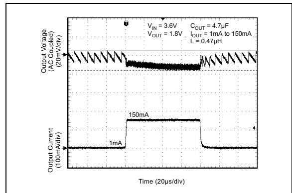
FIGURE 2-23: Load Transient.
