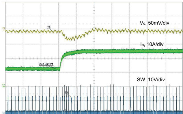
Fig. 46 - Load Step, 6 A to 12 A, 1 A/ \mu\text{s} , t = 10\text{ }\mu\text{s/div}
