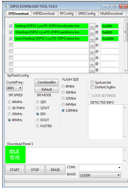
Figure 2-3. Flashing Configuration
