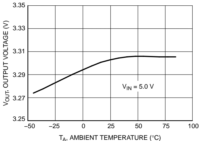
Figure 33. NCP1550SN33T1 Output Voltage versus Ambient Temperature
