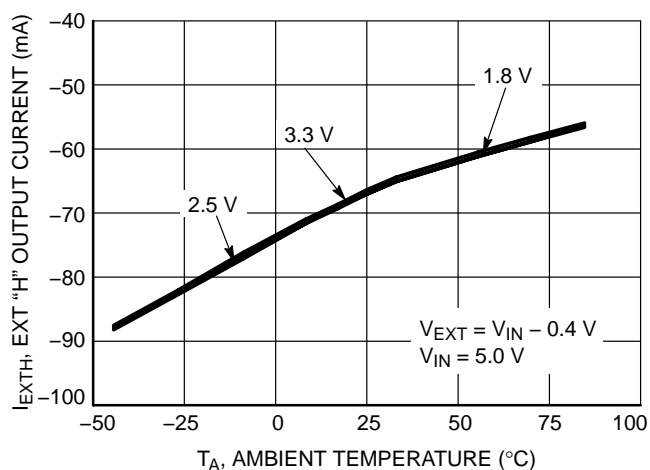
Figure 36. NCP1550 EXT "H" Output Current versus Ambient Temperature
