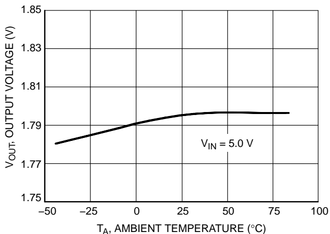
Figure 35. NCP1550SN18T1 Output Voltage versus Ambient Temperature
