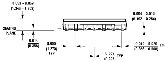
14-Lead Small Outline Molded Package (M) Order Number DM74LS21M NS Package Number M14A
