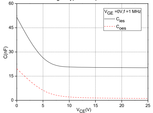
Fig.4 Capacitance Characteristics
