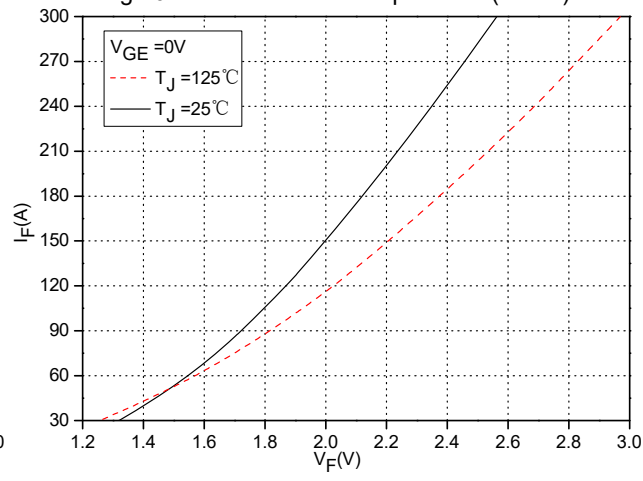
Fig.12 Forward Characteristics (Diode, 3-Level)
