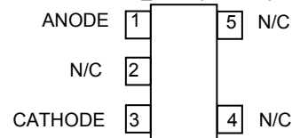
LM4041_H5 (SC70-5)
