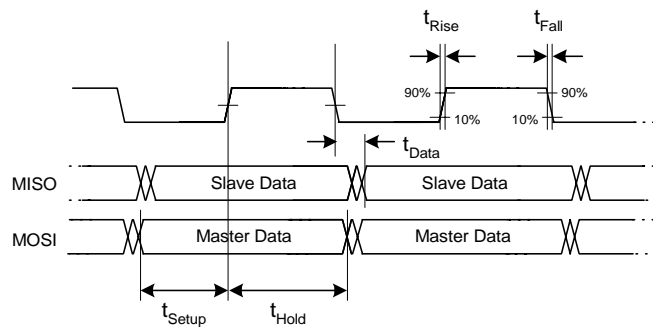
Figure 25: SPI timing
