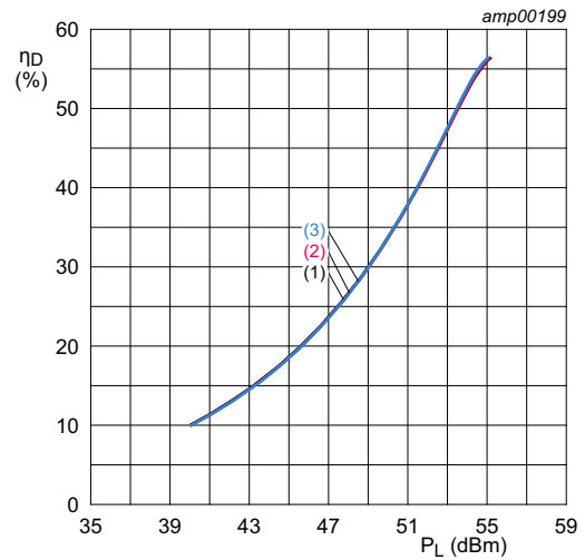
V_{DS} = 28\text{ V}; I_{Dq} = 1600\text{ mA}; t_p = 100\text{ }\mu\text{s}; \delta = 10\text{ }\% . (1) f = 2110\text{ MHz} (2) f = 2140\text{ MHz} (3) f = 2170\text{ MHz}
