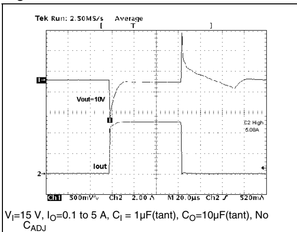
Figure 31. Load Transient
