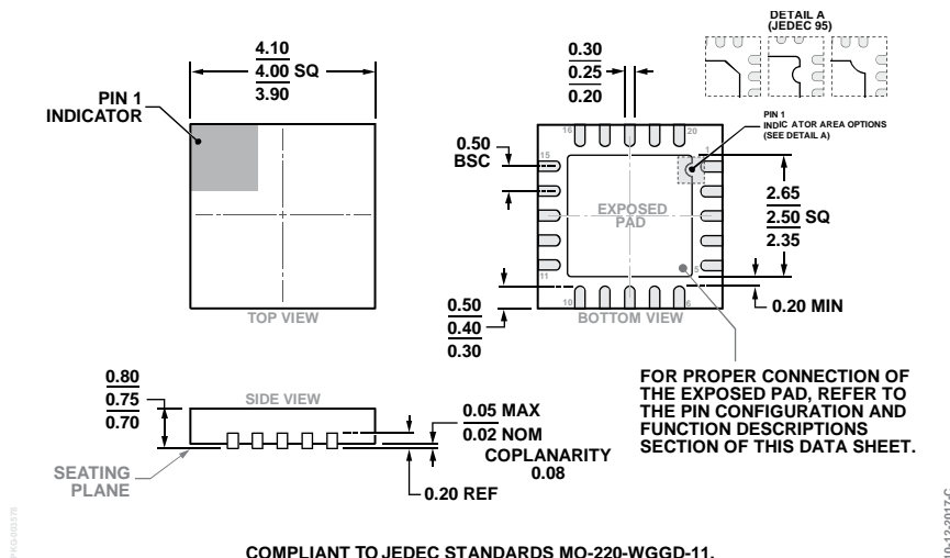
Figure 22. 20-Lead Lead Frame Chip Scale Package (LFCSP) 4 mm x 4 mm Body and 0.75 mm Package Height (CP-20-10) Dimensions shown in millimeters
