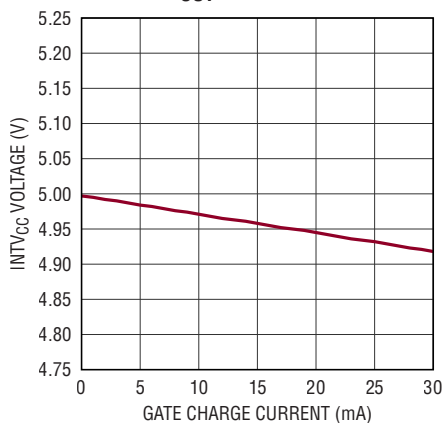
INTV CC Voltage vs Gate Charge Current V_{OUT} = 5\text{V}
