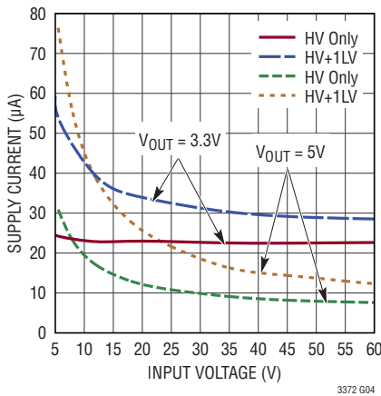
Burst Mode Quiescent Current vs V_{IN}
