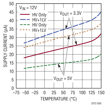
Burst Mode Quiescent Current vs Temperature
