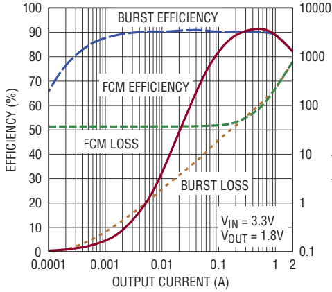
2A Buck Efficiency and Power Loss vs Output Current
