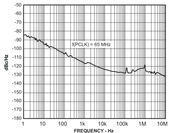
Figure 6-17. Phase Noise
