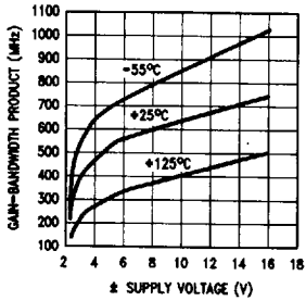
Gain-Bandwidth Product
