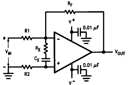
Noise-Gain Compensation
