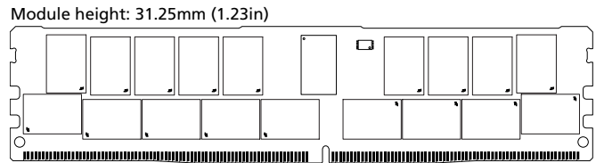
Figure 2: 288-Pin RDIMM (R/C-B2)
