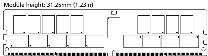
Figure 2: 288-Pin RDIMM (R/C-B2)
