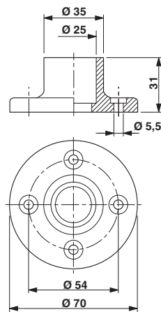
Dimensioned drawing
