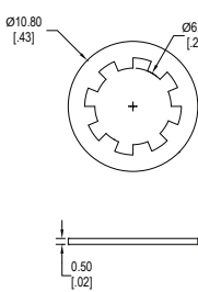
Lock Washer
