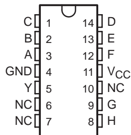
54AC11030 ... J PACKAGE 74AC11030 ... D OR N PACKAGE (TOP VIEW)
