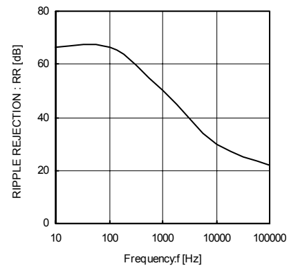
Fig. 7 Ripple Rejection
