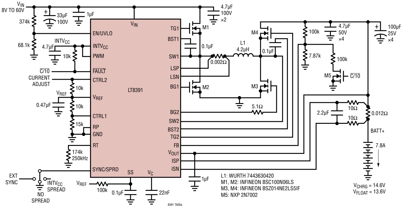
97% Efficient 8A Buck-Boost SLA Battery Charger
