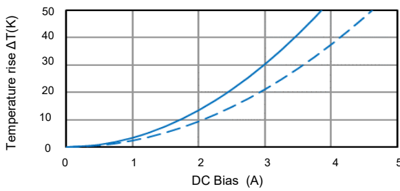
[ ▲ETQP5M470YSC ]
