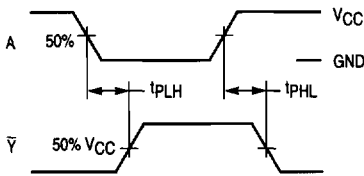
Figure 1. Switching Waveforms
