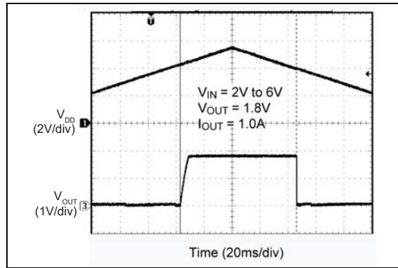
FIGURE 2-42: V_{DD} UVLO Thresholds.
