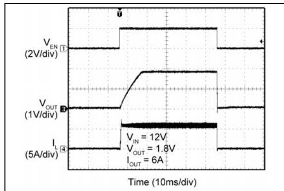
FIGURE 2-40: Enable Turn-On/Turn-Off.
