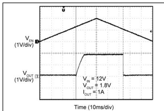
FIGURE 2-41: Enable Thresholds.
